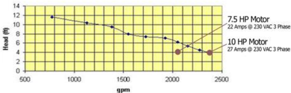
Riverflow Pump Curve NSF J-00030977
